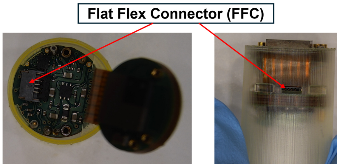
Figure S2: Custom PCB electronics in 3D-printed package facilitating alignment of the flat flex connector (FFC) with a sensor port.
