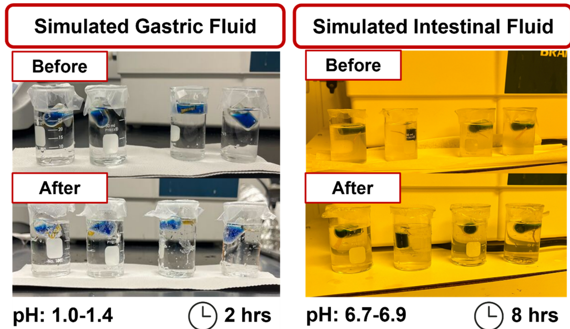
Figure S3: Capsule sealing integrity tests with die filled capsules in simulated gastric (left) and intestinal (right) fluid.
