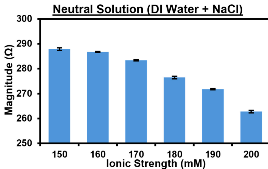
Figure S1: Magnitude impedance ( f = 10\text{kHz} ) of PEDOT:PSS electrodes ( N = 3 ) recorded at increasing ionic strengths a pH neutral solution.
