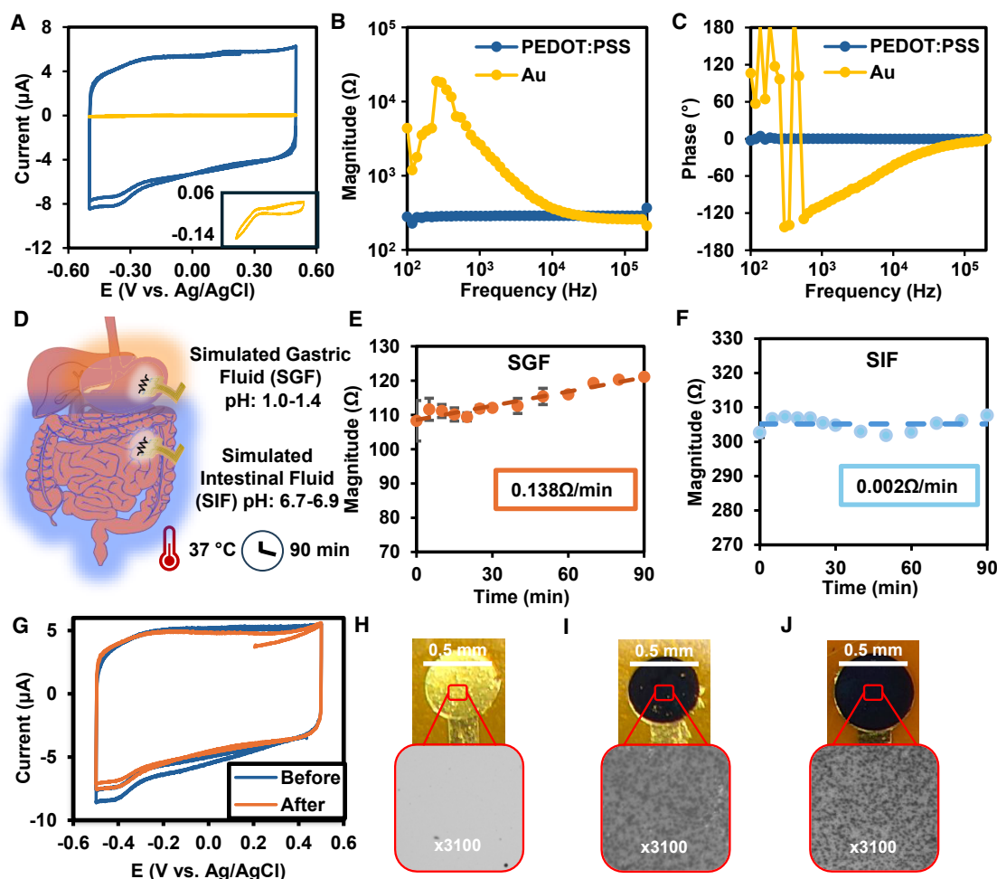
Figure 3. Bioimpedance sensor characterization
